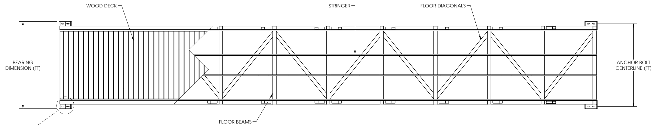
BRIDGE PLAN
